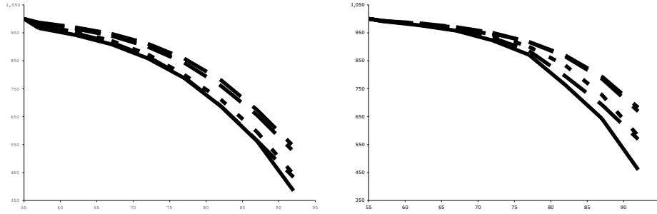
FIGURE 6. Number of survivors of an initial cohort of 1,000 male (left) and female lives at age 55, based on the Society of Actuaries TSA Reports for 1951, 1961, 1971, 1981, and 1991 on group annuity experience, without adjustments.
