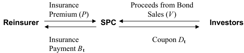
FIGURE 1. Mortality Bond Cash Flow Diagram.
