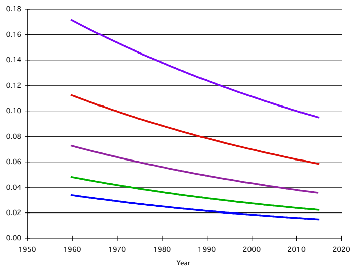
FIGURE 7. Male Group Annuity Mortality, predicted forces of mortality based on 6-parameter log-link model and TSA Reports 1951 - 1992. The top curve is the force of mortality for age 85, the one just below it is for age 80, then 75, 70 and the bottom curve is for age 65. The greatest improvement (steepest slope) is at age 85.
