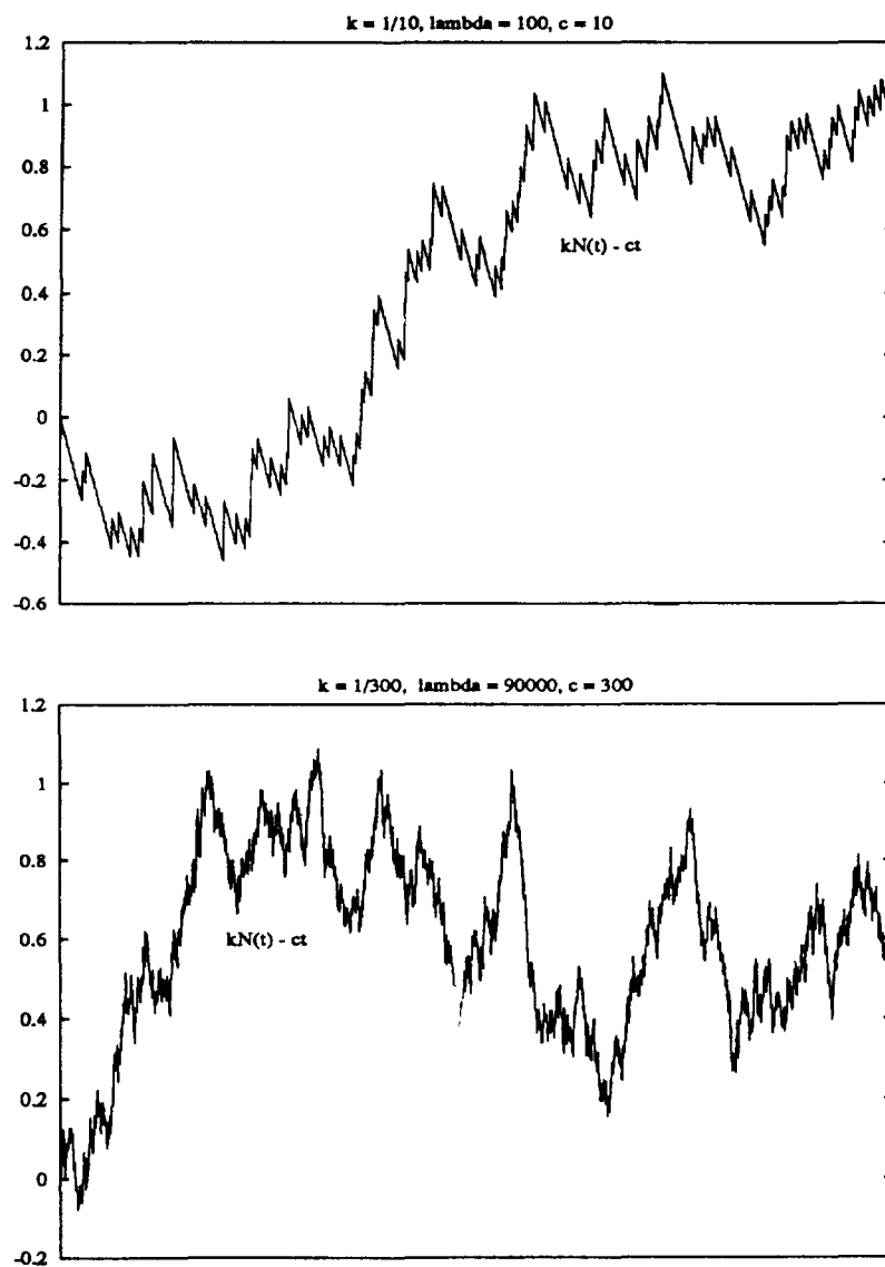
FIGURE 1 SAMPLES PATHS OF TWO SHIFTED POISSON PROCESSES WITH \mu = 0 AND \sigma^2 = 1
